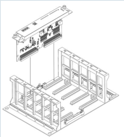
Model XNLC Diagram of an `Class X' Intelligent Notification Loop Card mounted to a Siemens Card Cage
