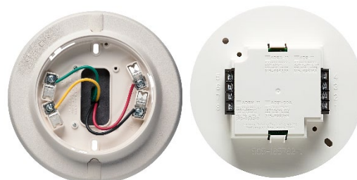
Model SBGA-34 (Front & Back View)
