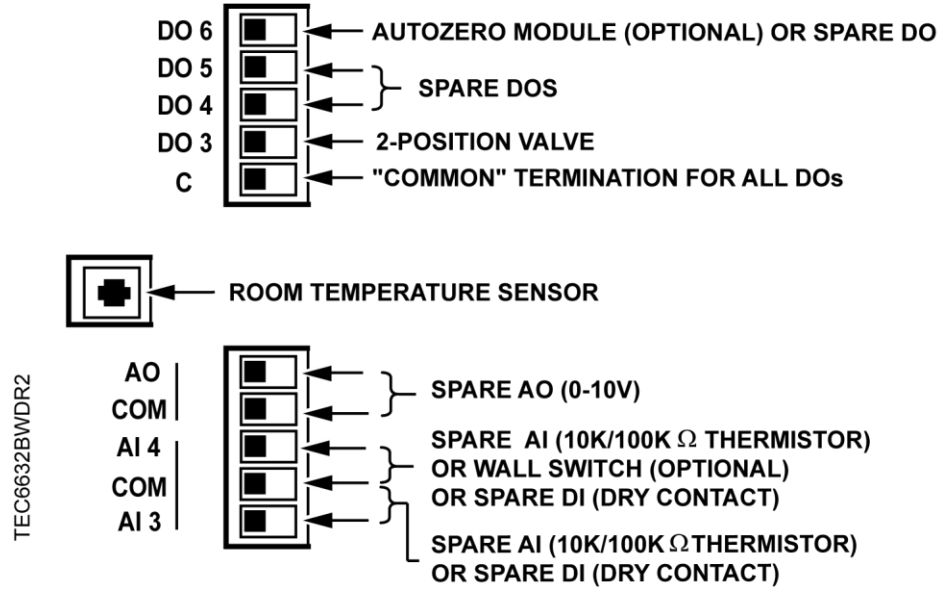
Application 6632 VAV with Baseboard Radiation Wiring Diagram.
