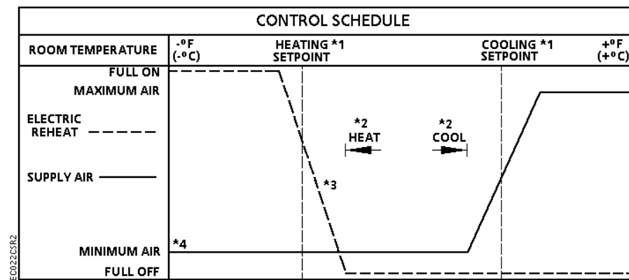
Application 6632 with Electric Heat Control Schedule.
