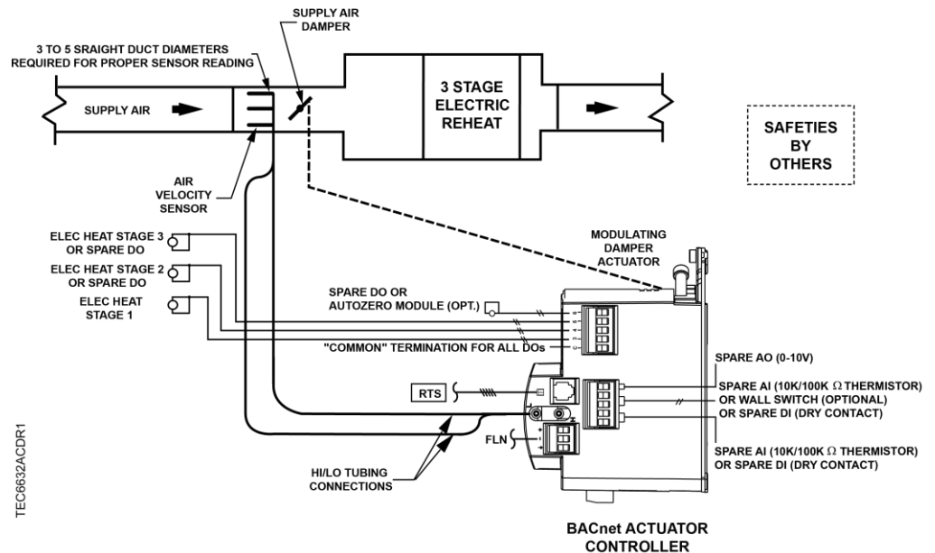
Application 6632 with Electric Heat Control Diagram.
