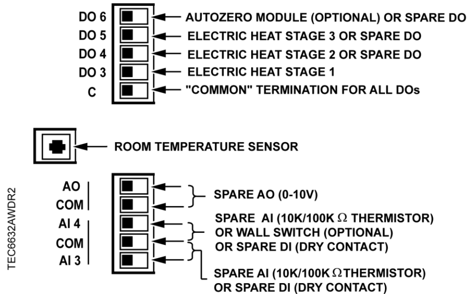
Application 6632 VAV with Electric Heat Wiring Diagram.
