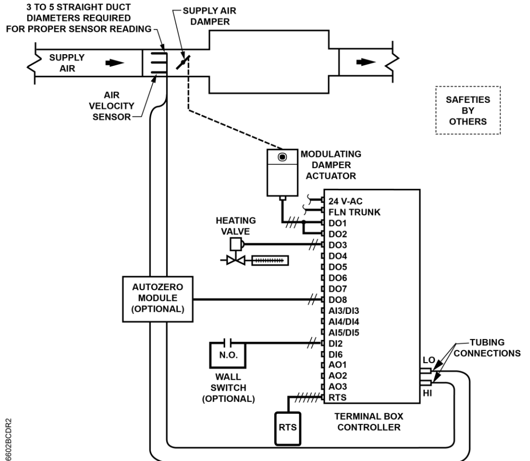
Application 6602 - VAV with Baseboard Radiation.
