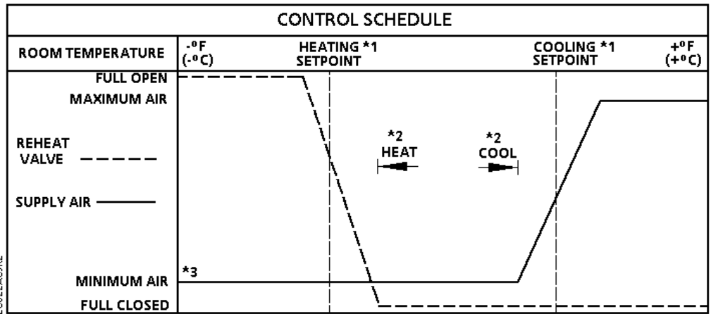
Application 6602 Control Schedule.
