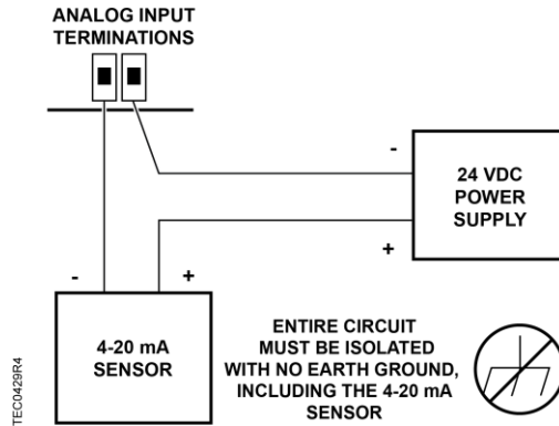
TEC042BR4 Wiring for AI with a 4 to 20 mA Sensor.
