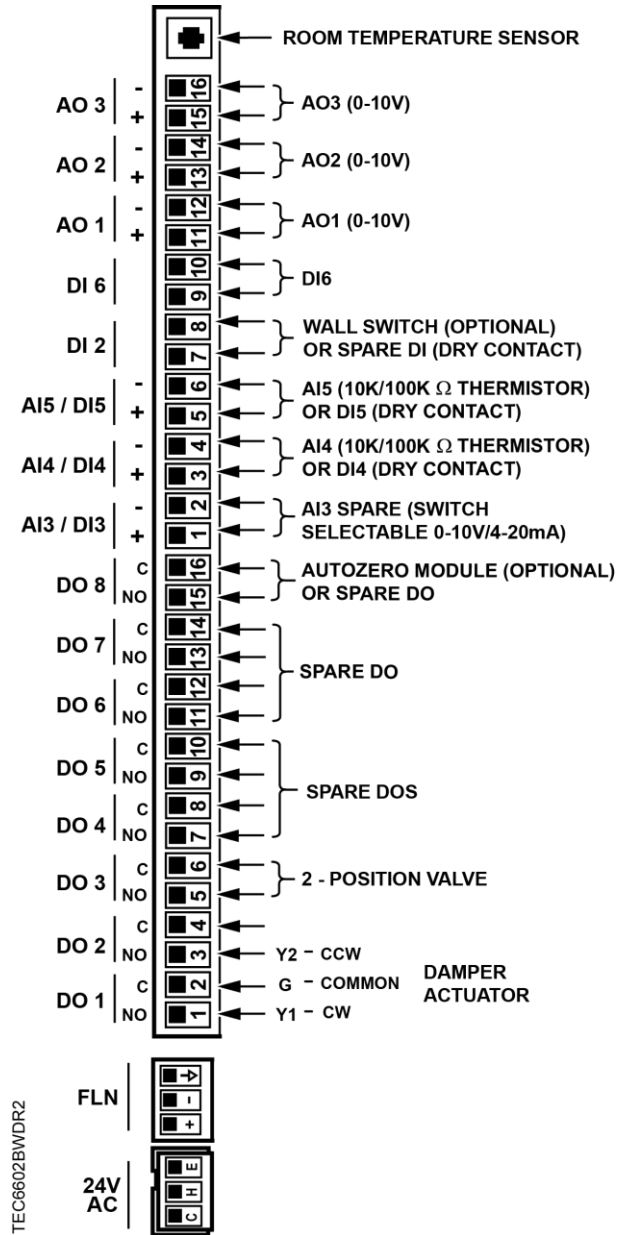
Application 6602 – Variable Air Volume with Baseboard Radiation.
