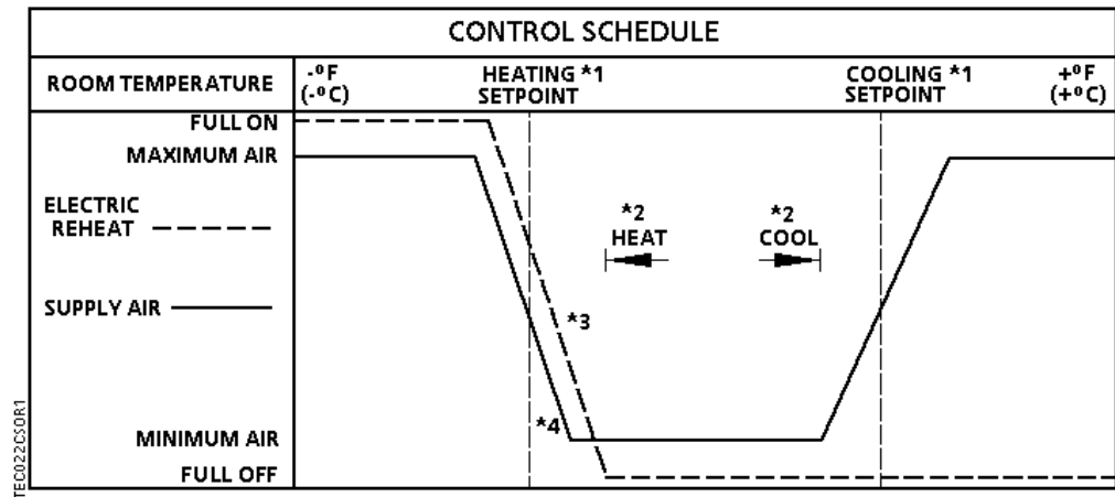
Application 6602 Heating Mode Control Schedule.
