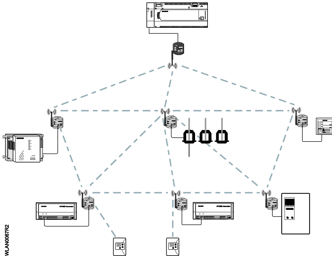
Figure 2. WFLN with WRTs.
