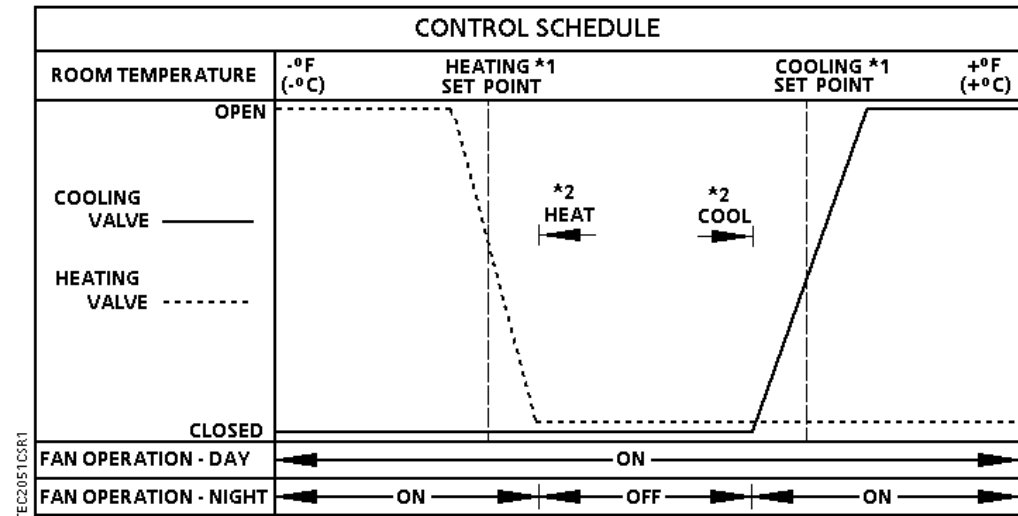
Application 2051 Control Schedule.
