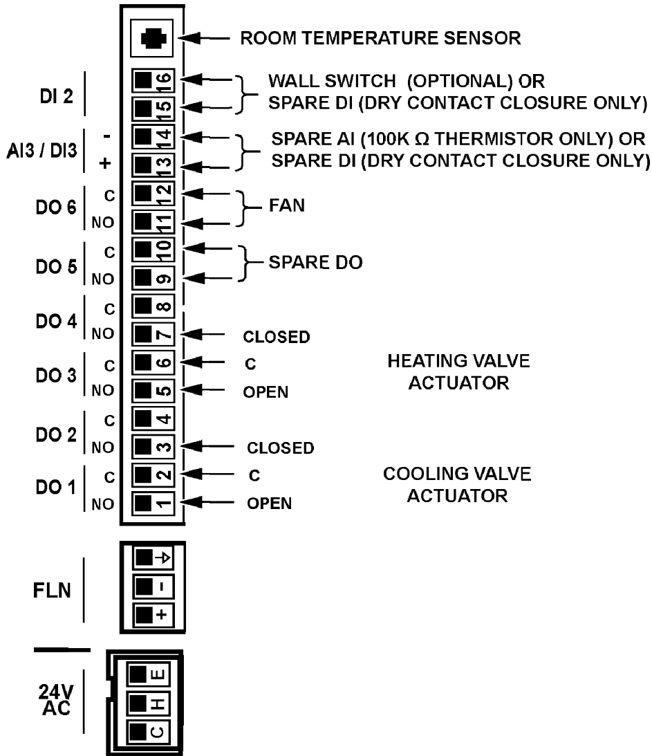
Application 2051 – Fan Coil Unit Cooling and Heating.
