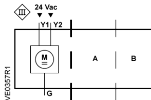
Figure 4. Wiring Designations.
