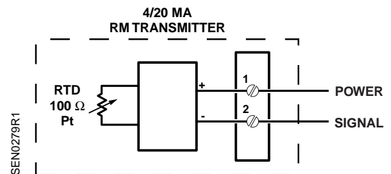
Figure 3. Sensor Terminal Block Wiring.
