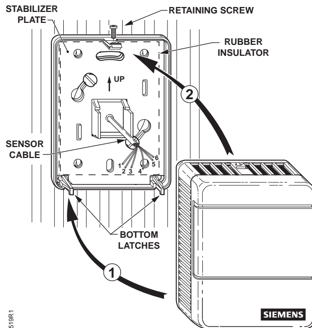
Figure 2. Drywall Mounting (No Rough-in).
