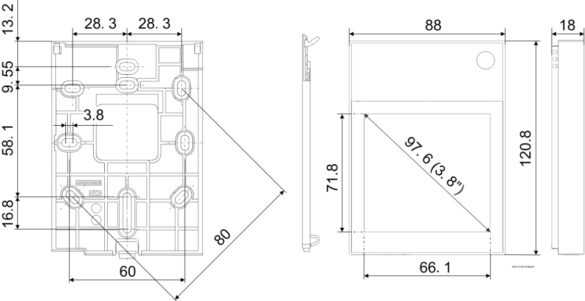
Fig. 4: Dimension drawing
