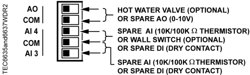
Application 6635/6637 VAV Series Fan or Parallel Fan and Hot Water Heat Wiring Diagram.
