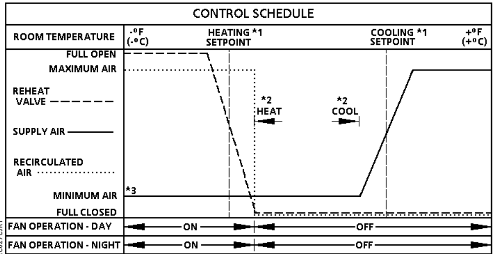
Application 6637 Control Schedule.
