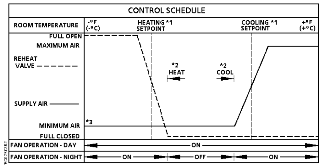
Application 6635 with Hot Water Heat Control Schedule.
