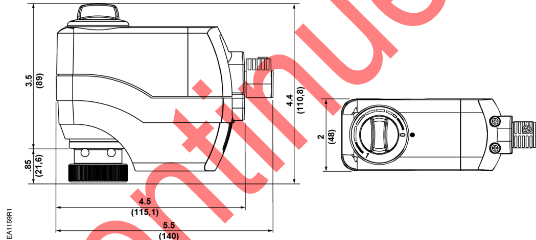
Figure 7. SSC61.5U Series Actuator Dimensions in Inches (Millimeters).
