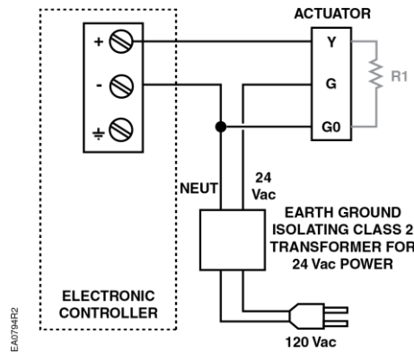
Figure 4. SSC61.5U Wiring.
