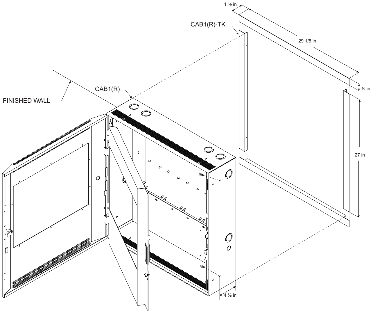
Figure 1 Typical Trim Kit Installation
