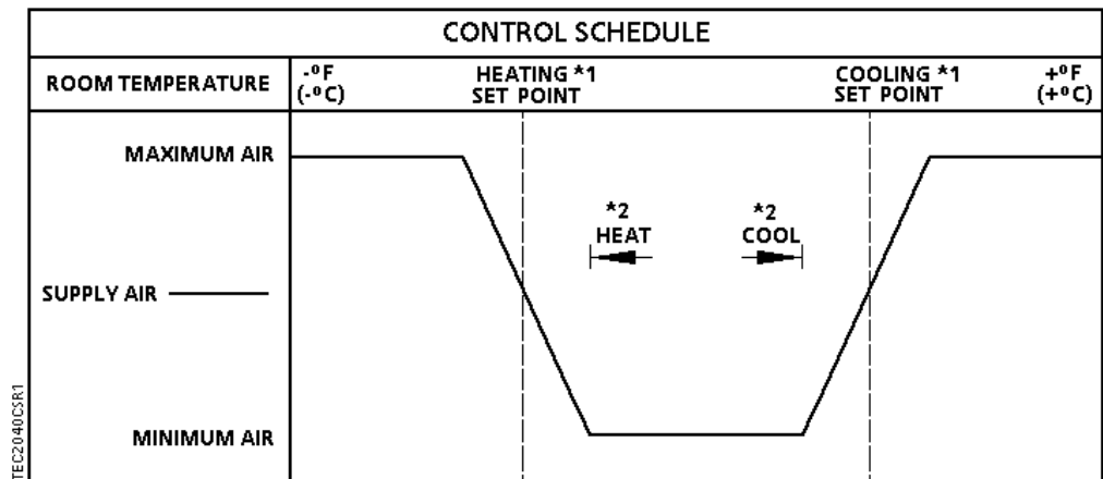
Application 6540 Control Schedule.
