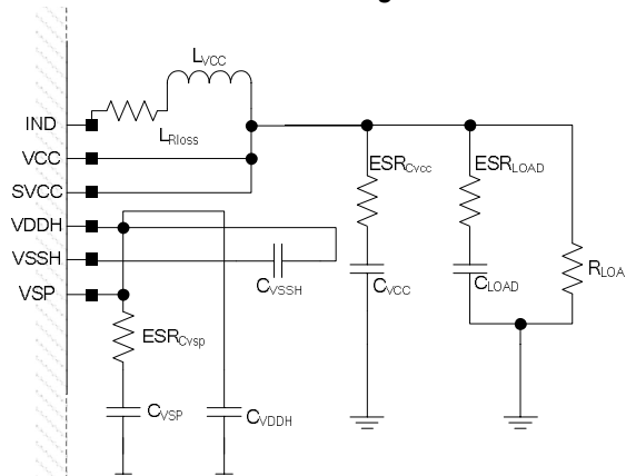
Figure 2 VCC supply external connections
