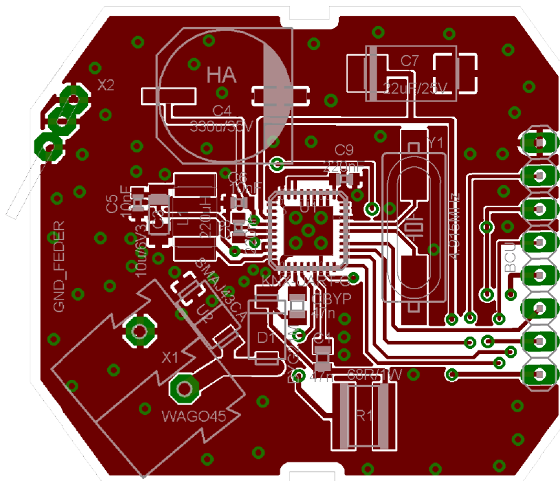
Figure 13 Layout Topview
