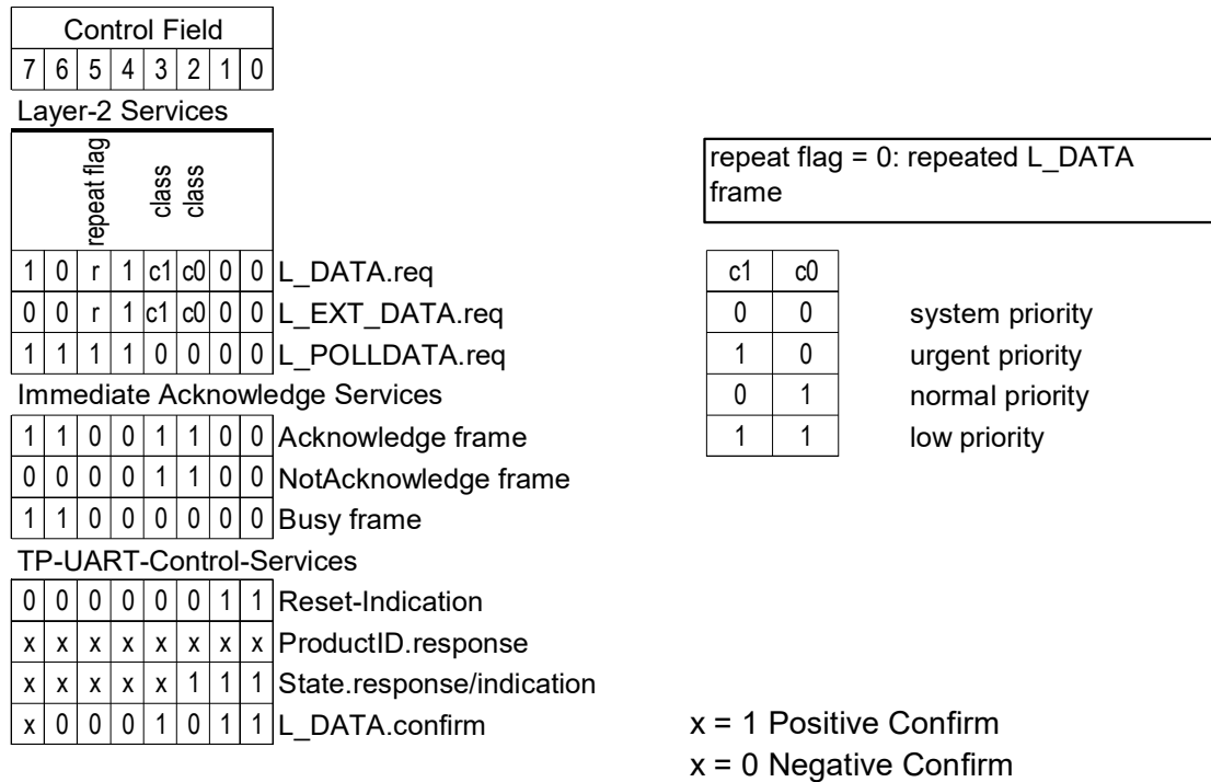
Fig. 25: Control Field
